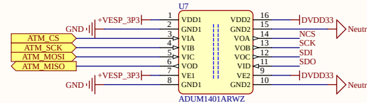
SPI INTERFACE ISOLATED
